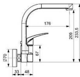
SINK MIXER WALL EVİYE BATARYASI ÜSTTEN APLİKE
