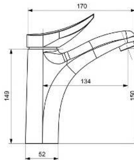
WASHBASIN MIXER M LAVABO BATARYASI ORTA
