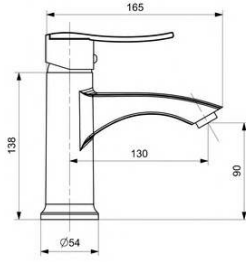
WASHBASIN MIXER LAVABO BATARYASI
