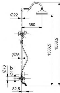
LONG BATH FAUCET ROBOT BANYO BAT TAKIM
