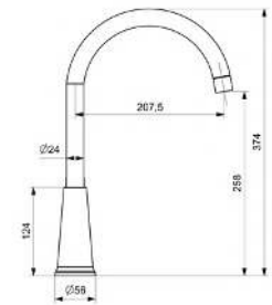
SINK MIXER EVİYE BATARYASI
