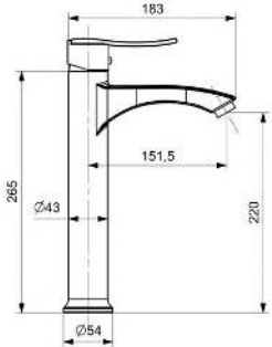
WASHBASIN MIXER L LAVABO BATARYASI ÇANAK
