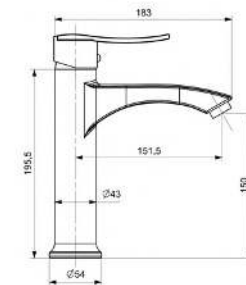
WASHBASIN MIXER M LAVABO BATARYASI ORTA
