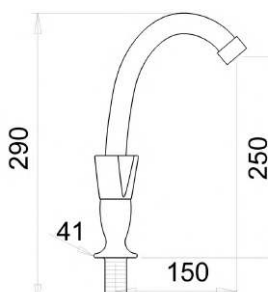
BRIDGE FAUCET KÖPRÜ BATARYASI
