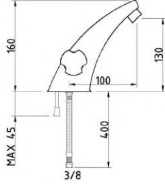
WASHBASIN FAUCET LAVABO BATARYASI
