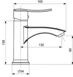
WASHBASIN MIXER LAVABO BATARYASI
