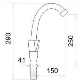
BRIDGE FAUCET KÖPRÜ BATARYASI
