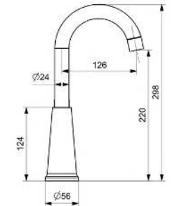
WASHBASIN MIXER S LAVABO BATARYASI BORULU
