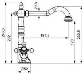
SINK FAUCET EVYE BATARYASI
