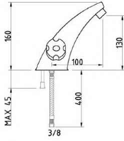
WASHBASIN FAUCET LAVABO BATARYASI
